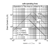
RATING AND CHARACTERISTIC CURVES (4N65F)
