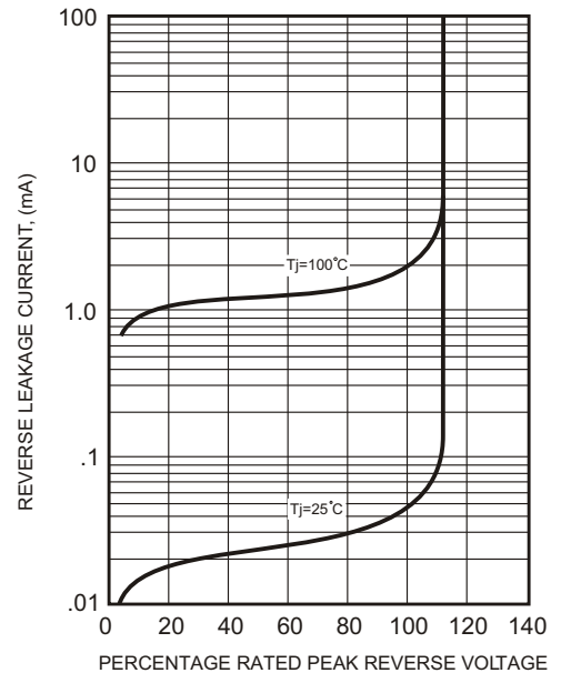
FIG.5 - TYPICAL REVERSE
