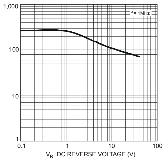
FIG.4-TYPICAL JUNCTION CAPACITANCE
