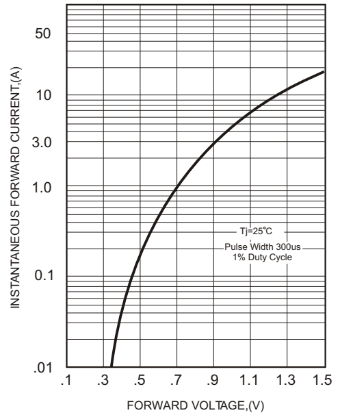
FIG.2-TYPICAL FORWARD
