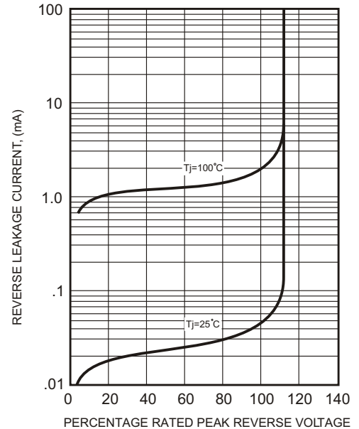
FIG.5 - TYPICAL REVERSE
