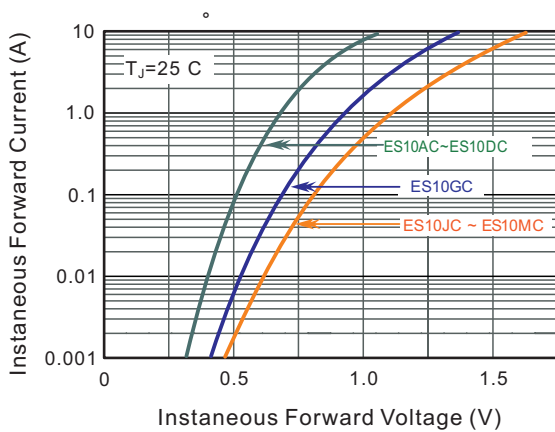
FIG.3-TYPICAL FORWARD CHARACTERISTICS
