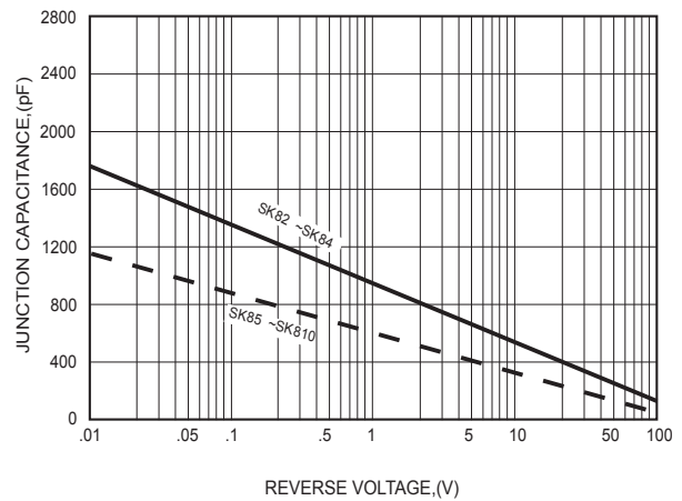
FIG.4-TYPICAL JUNCTION CAPACITANCE
