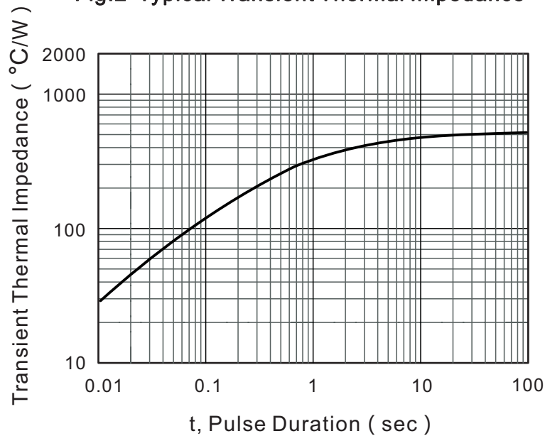
Fig.2 Typical Transient Thermal Impedance
