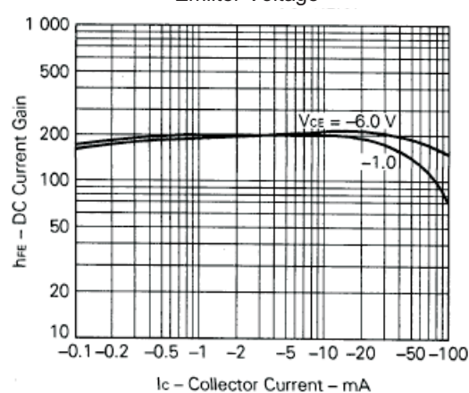
Fig.6 DC Current Gain vs. Collector Current
