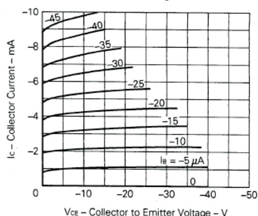
Fig.4 Collector Current vs. Collector to Emitter Voltage
