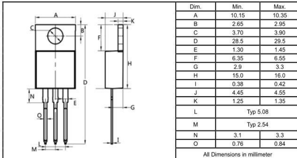
TO-220F
