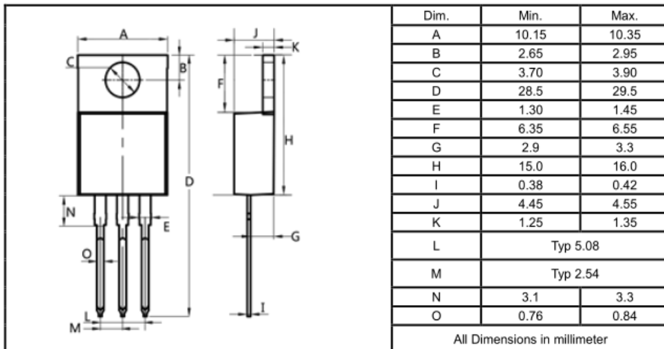
TO-220F
