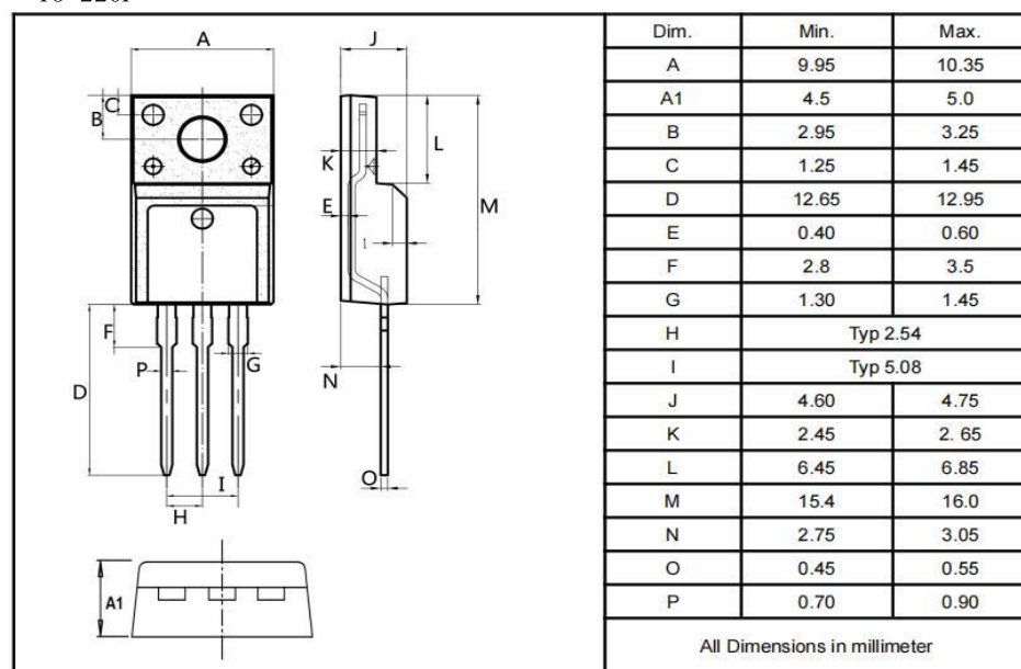
TO-220F
