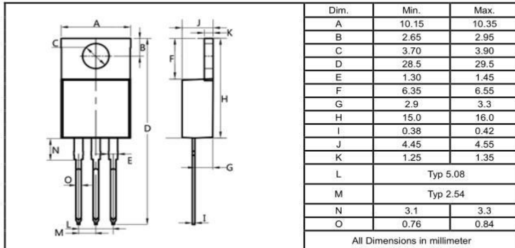
TO-220F
