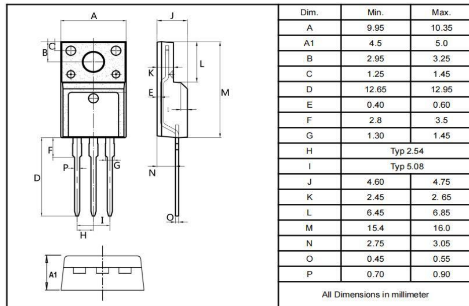
TO-220F
