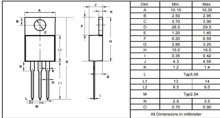
TO-220F
