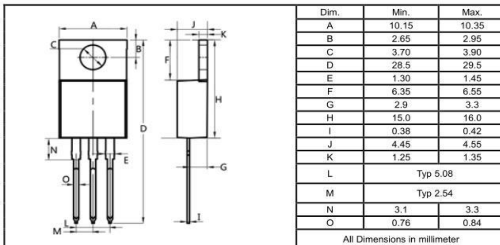
TO-220F
